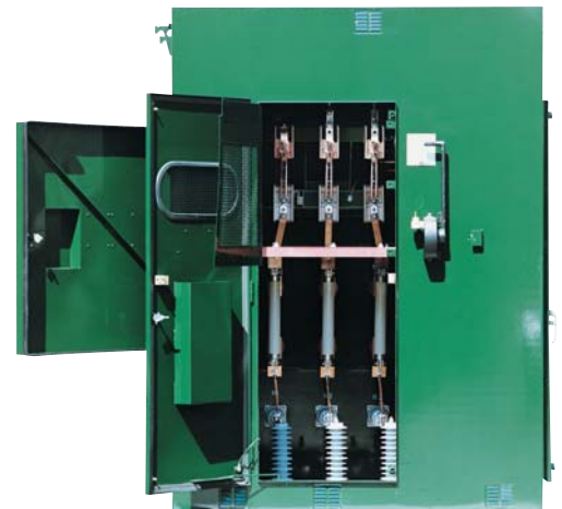
1500 KVA 25kV \Delta -600Y/347V Unitized Pad-Mount
